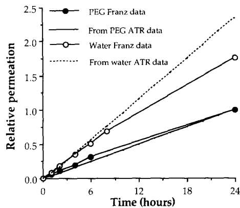
Fig. 3. Comparison of ATR derived simulated diffusion profiles with Franz cell diffusion profiles.
